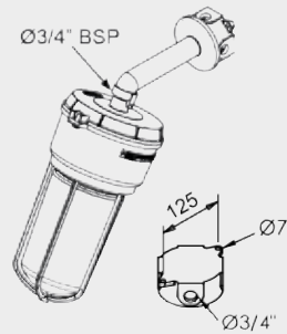
AY116 - Arandela 30°
